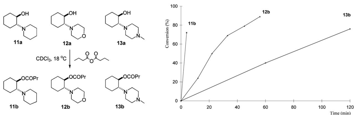
Figure 3. Acylation of amino alcohols influenced by electronic effects.
