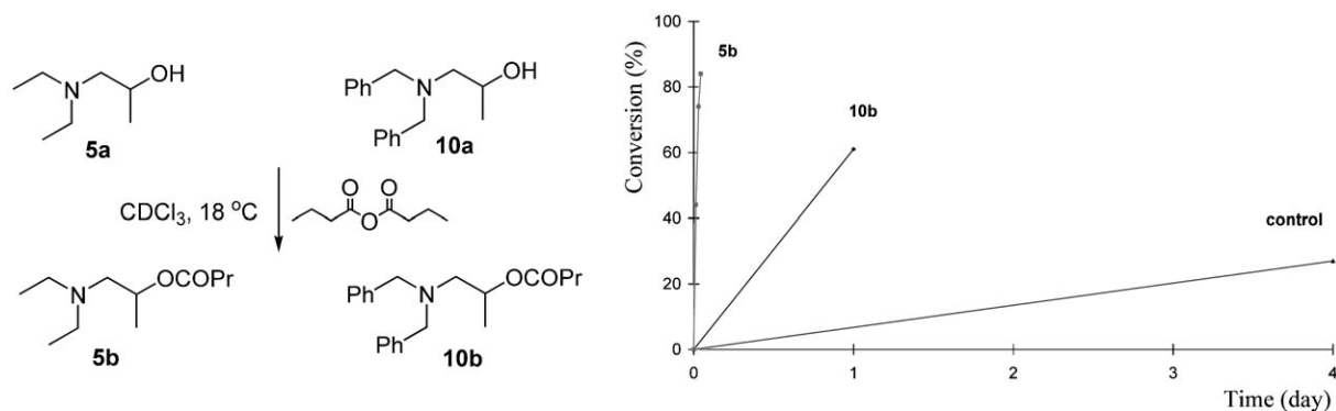
Figure 2. Acylation of amino alcohols influenced by steric effect (control: 1:1 mixture of 2-propanol/triethylamine).
