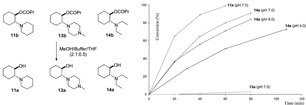
Figure 4. Methanolysis of amino esters ( 40^\circ\text{C} , \text{THF/MeOH} , buffer. Not shown: addition of 1 equivalent of TFA quenches the reaction altogether).
