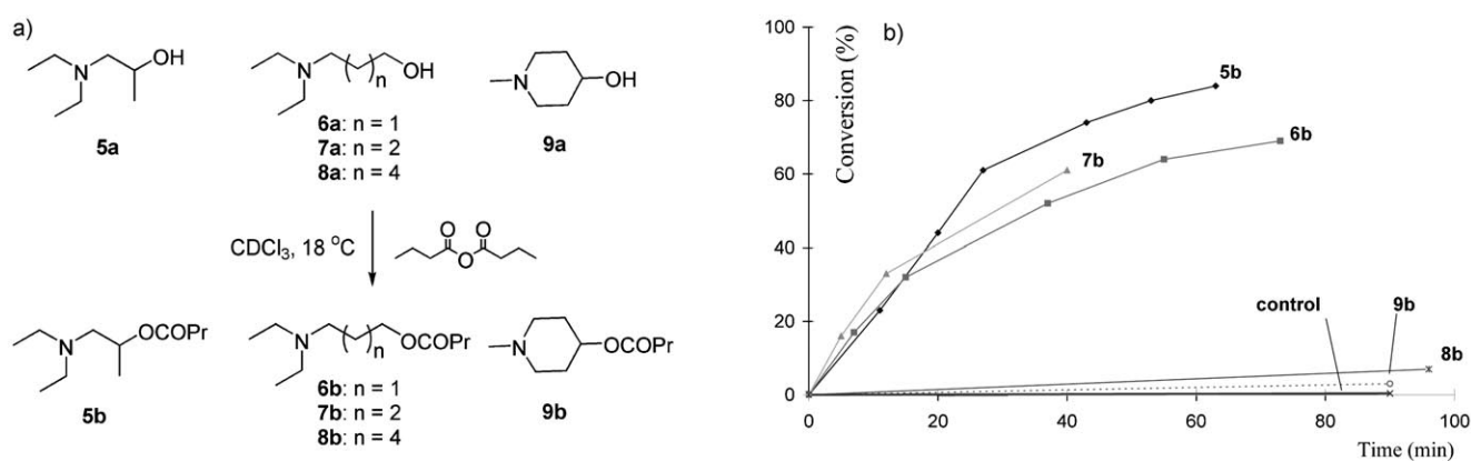
Figure 1. Acylation of amino alcohols influenced by spatial effects (18 °C, in \text{CDCl}_3 ; control: 1:1 mixture of 2-propanol/triethylamine).
